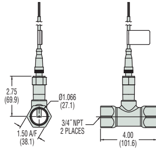
1" NPT Port
