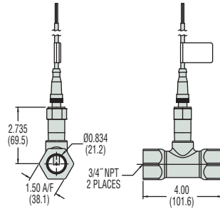
3/4" NPT Port
